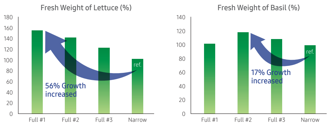
Figure 8. Performance of narrow and full LED spectrum
